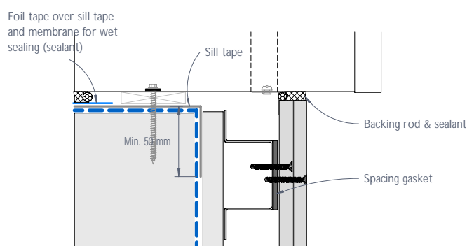
Figure 11: CEDRAL LAP meter box junction - Section
