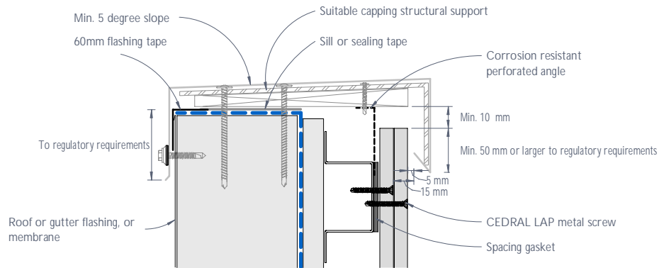
Figure 29: CEDRAL LAP typical capping detail
