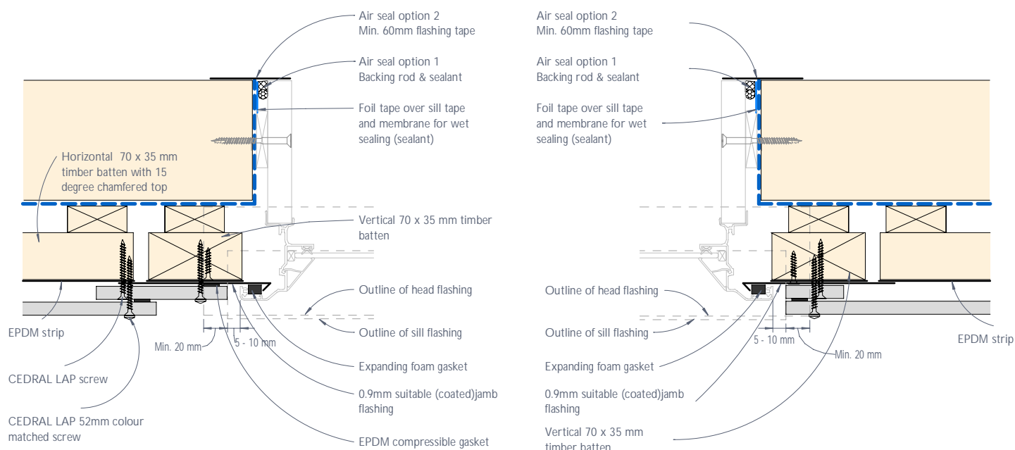
Figure 10: CEDRAL LAP window jamb junction or the like - Flush detail
