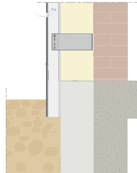
Figure 2: Ground Level
