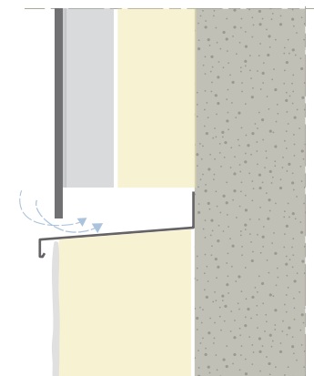
Figure 23: EQUITONE to render base detail
