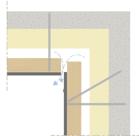
Figure 20: Soffit Detail
