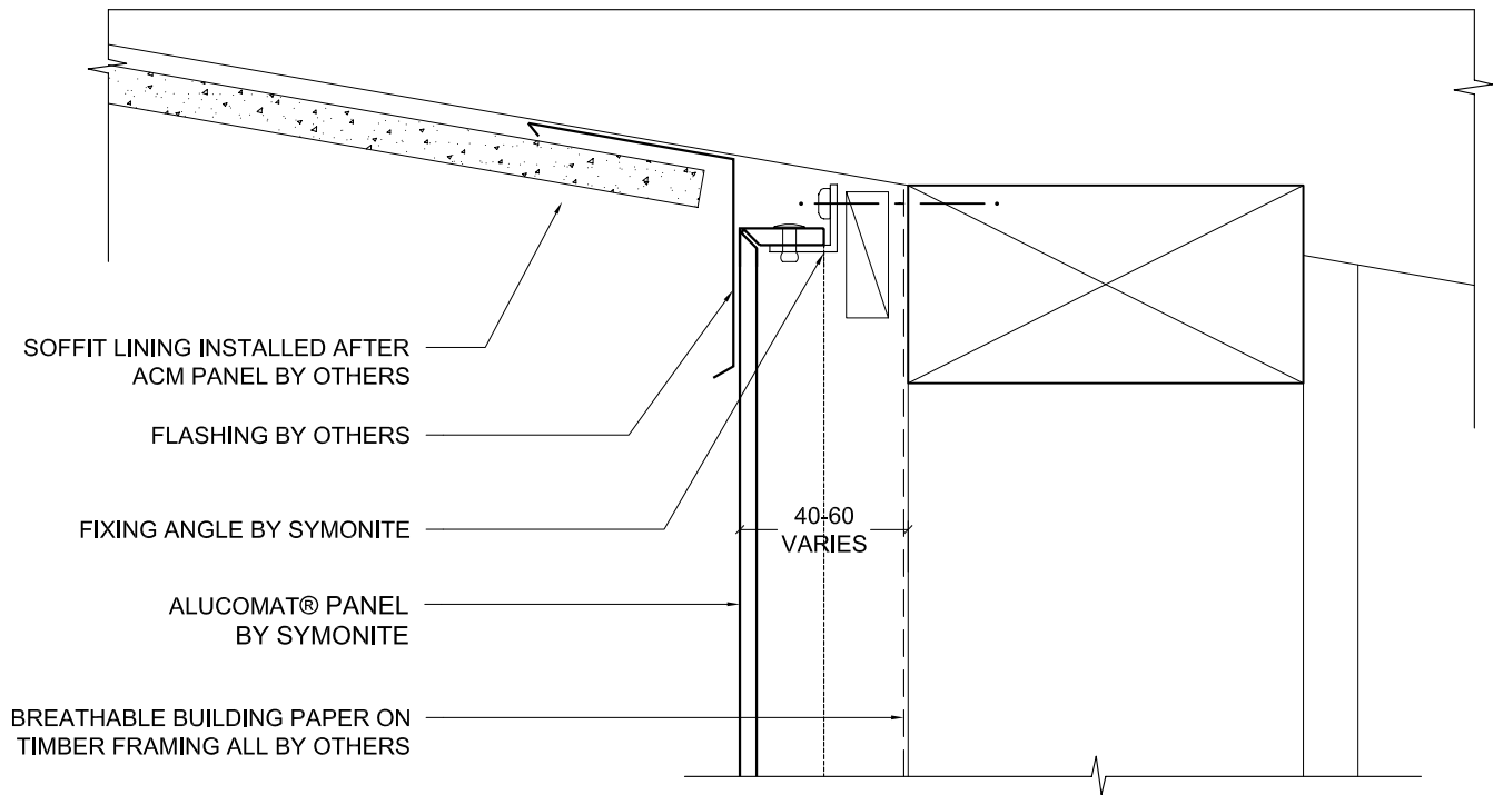
1 WALL / RAKING SOFFIT JUNCTION - OPTION 1 - 1:2 @ A4
