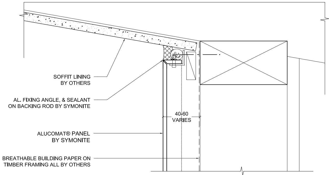
2 WALL / RAKING SOFFIT JUNCTION - OPTION 2 - 1:2 @ A4
