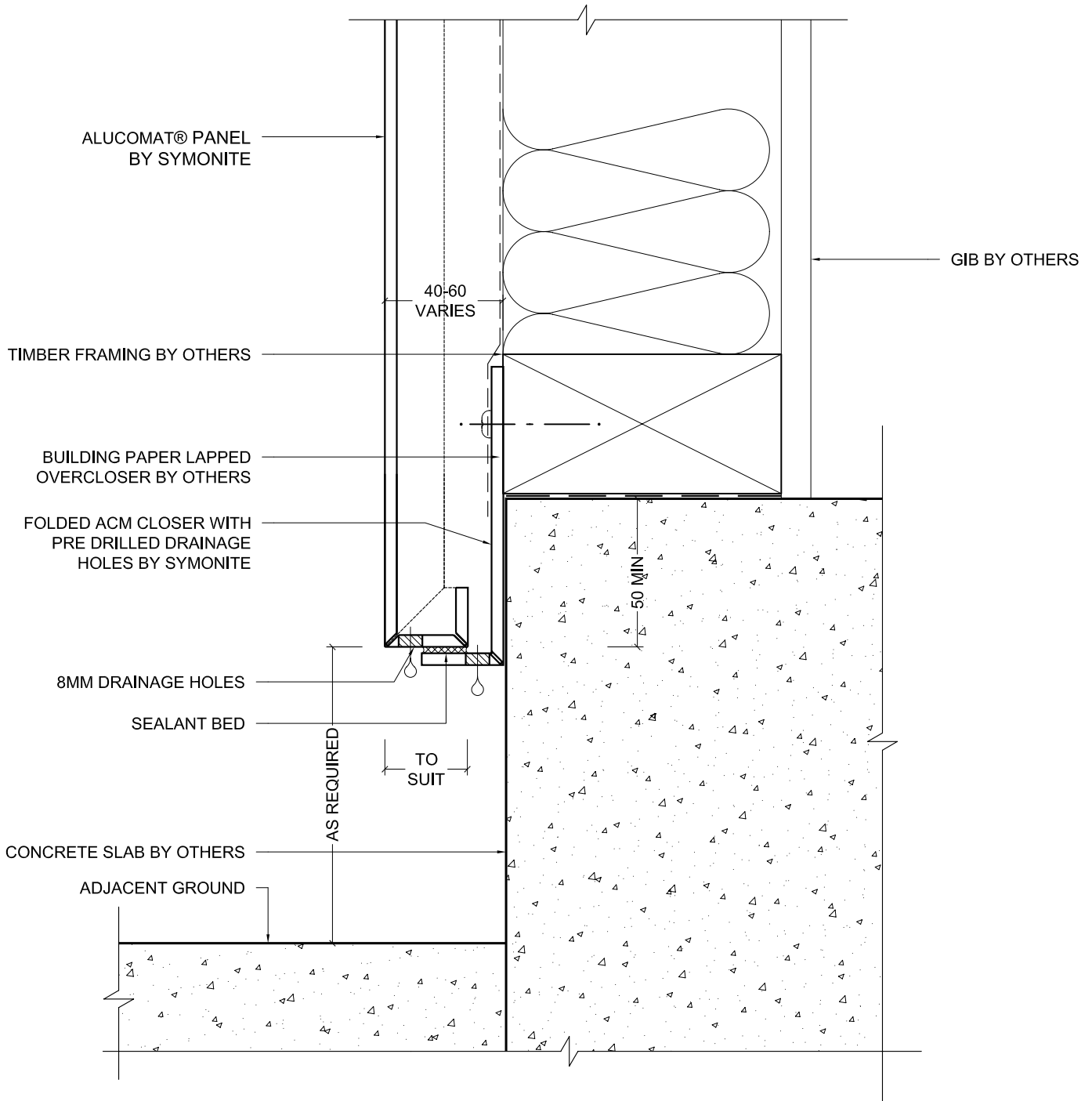
1 BASE DETAIL
