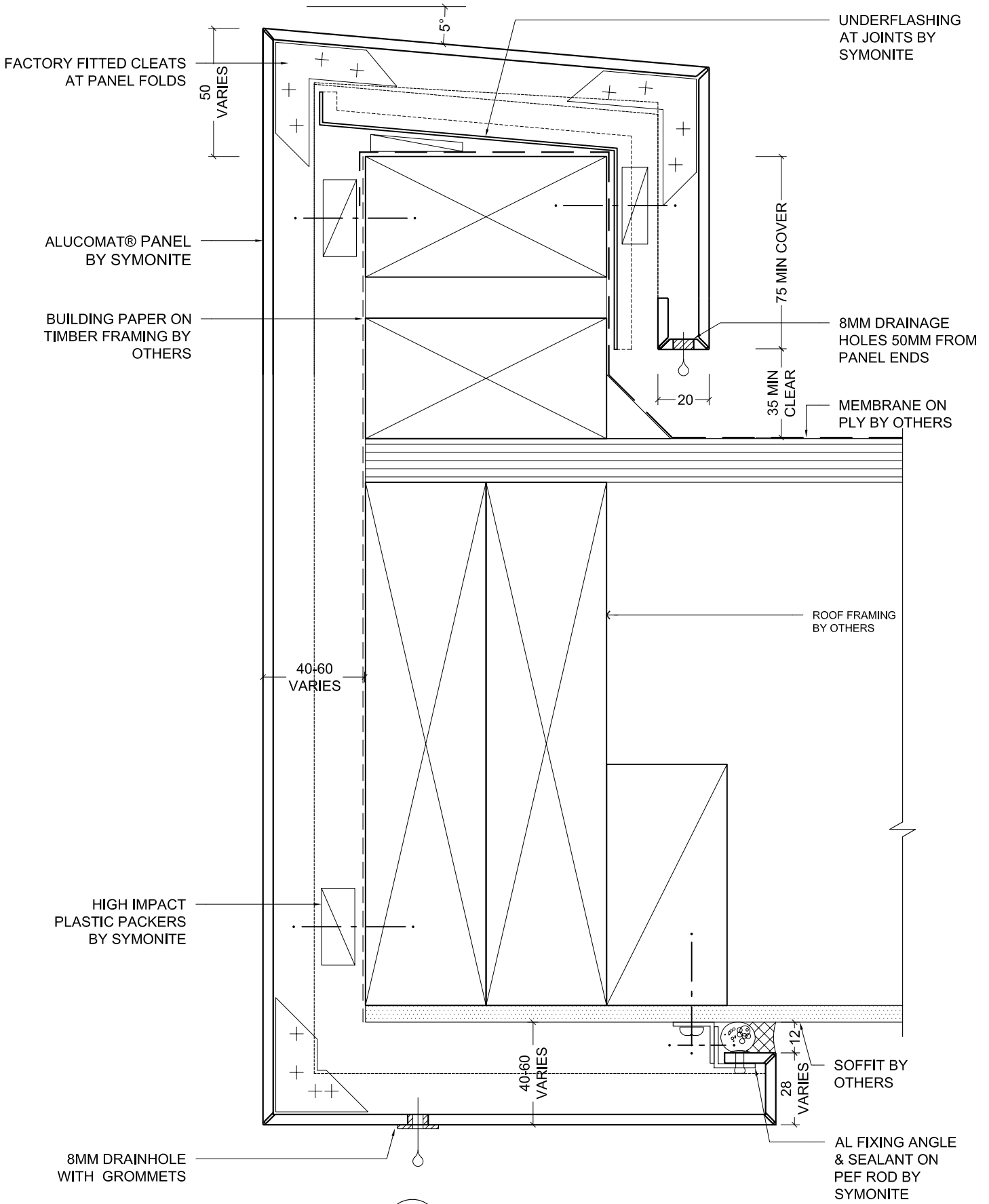
1 ACM FASCIA - SOFFIT BY OTHERS - 1:2 @ A4
