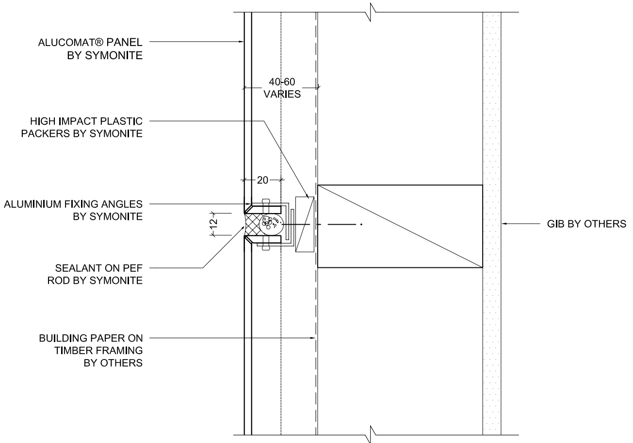
1 TYPICAL HORIZONTAL JOINT - 1:2 @ A4
